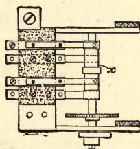
Fig. 350.—Aron Meter—Plan of Reversing Commutator
